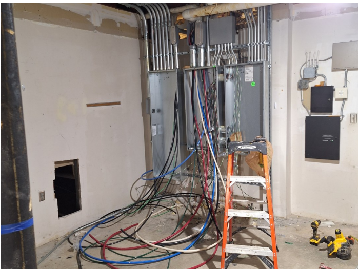
Pulling main feeder wire
